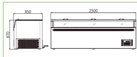
ZCD-L250S-S4 侧柜
